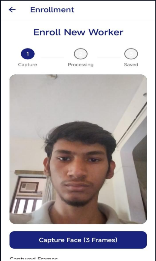
Face Enrollment
