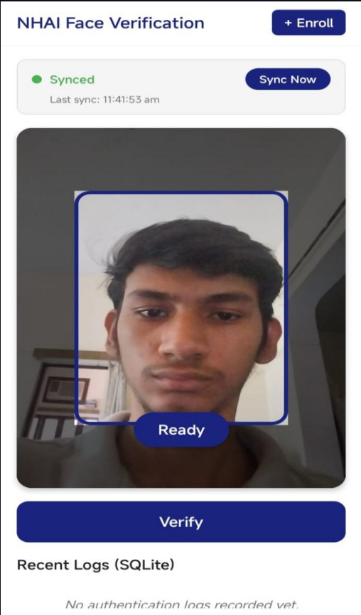
Authentication
