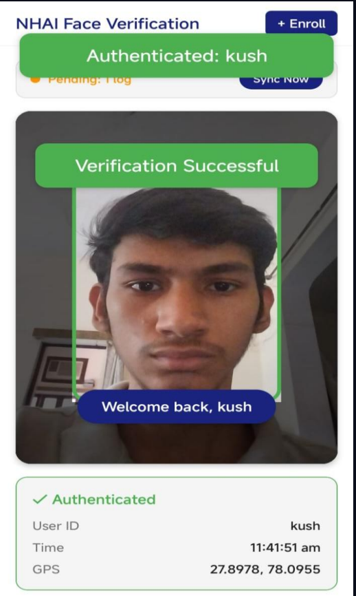
Auth Success
